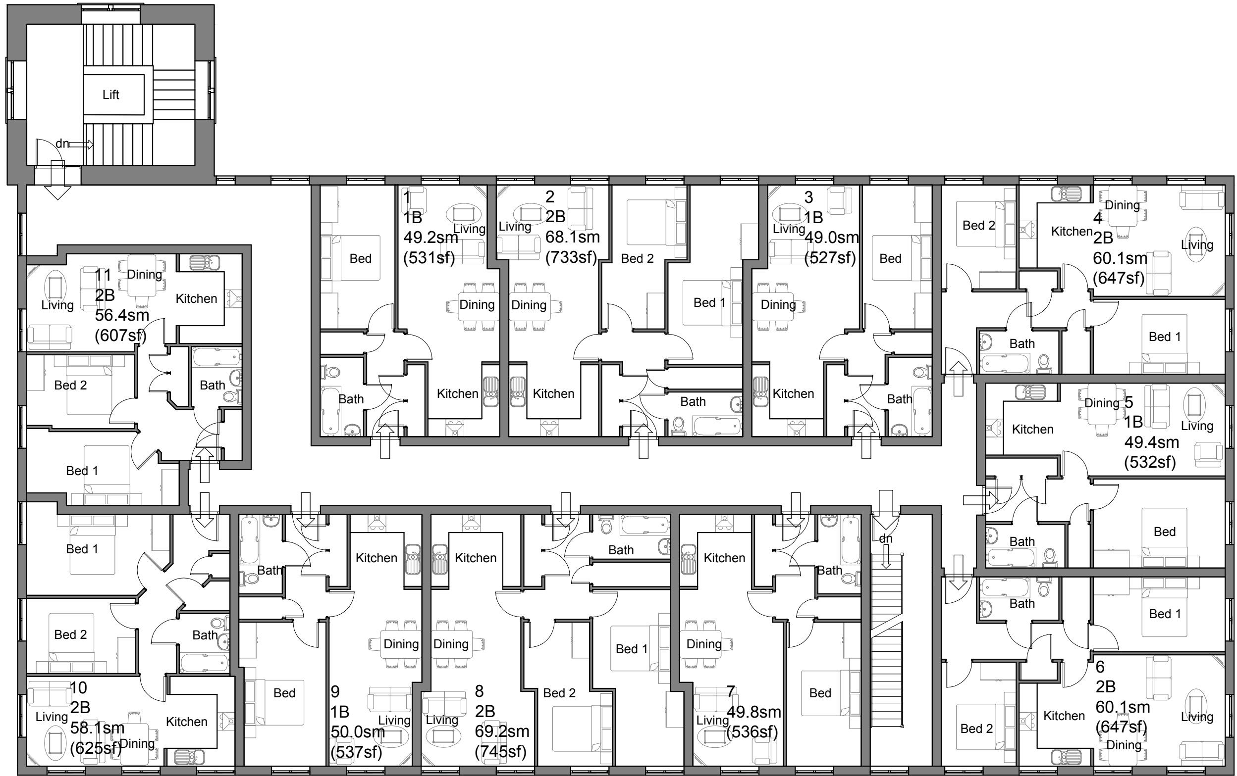
Mill First Floor
